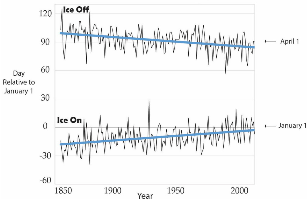
Lake Mendota Ice On and Off Dates, 1855-2023
