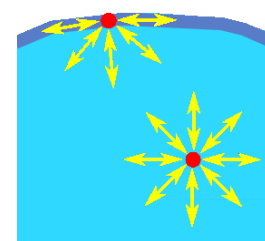
Water molecules (red) experience intermolecular forces (yellow).
